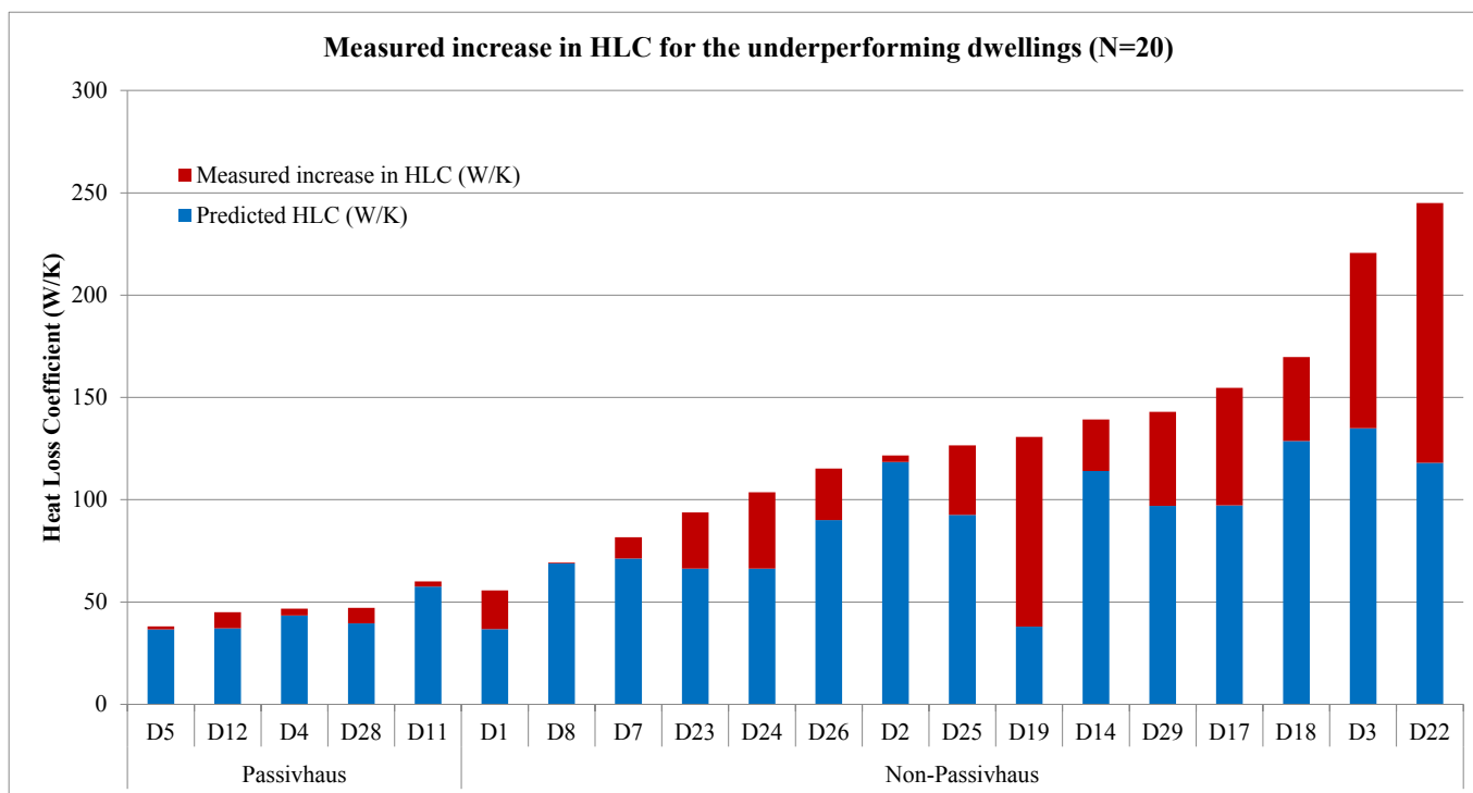
Figure 17. Measured increase in HLC in dwellings with co-heating test revealed performance gap.
